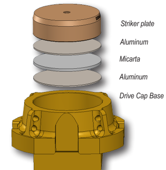
Drive Base Assembly
